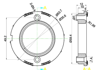
Installation Ring
