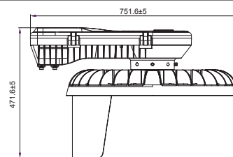
Side Shield
